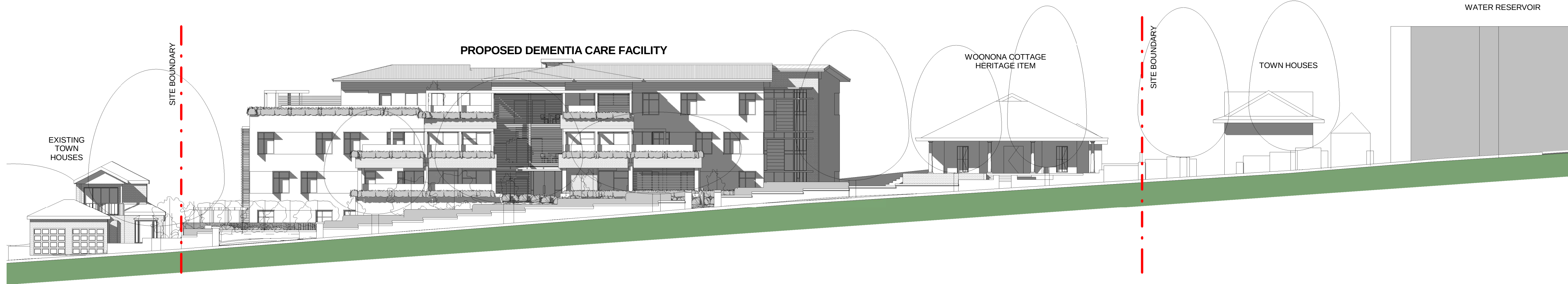
1 Woonona Avenue South Elevation (Facing West) 1 : 200
